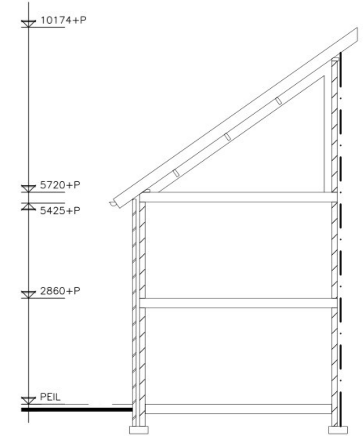
Doorsnede -bestand-
